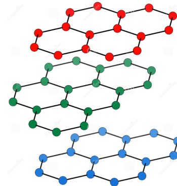
Hybridation sp^2
