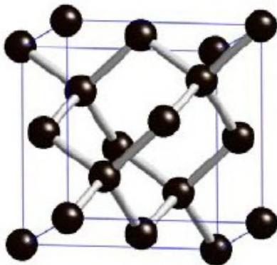
Hybridation sp^3
